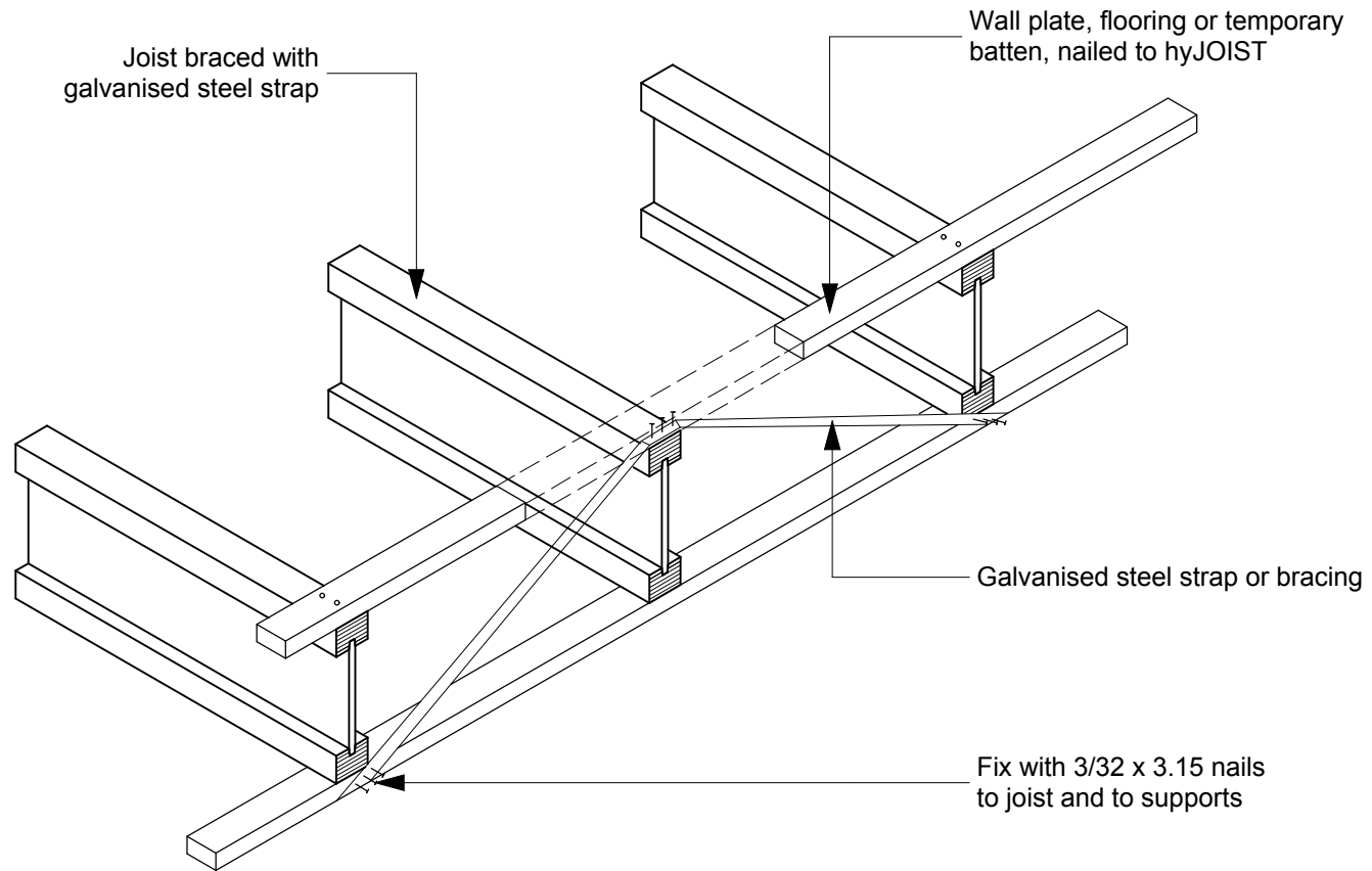
Detail F2 End restraint - using steel strap or bracing Scale: NTS May 2007
